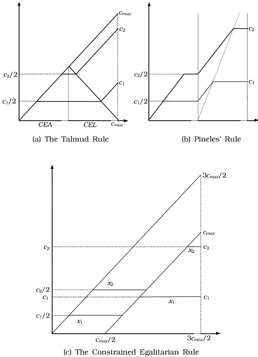
FIGURE 5 PARAMETRIC REPRESENTATIONS OF THREE RULES
